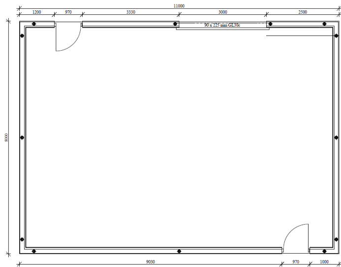
Figur 2. Garage plantegning
