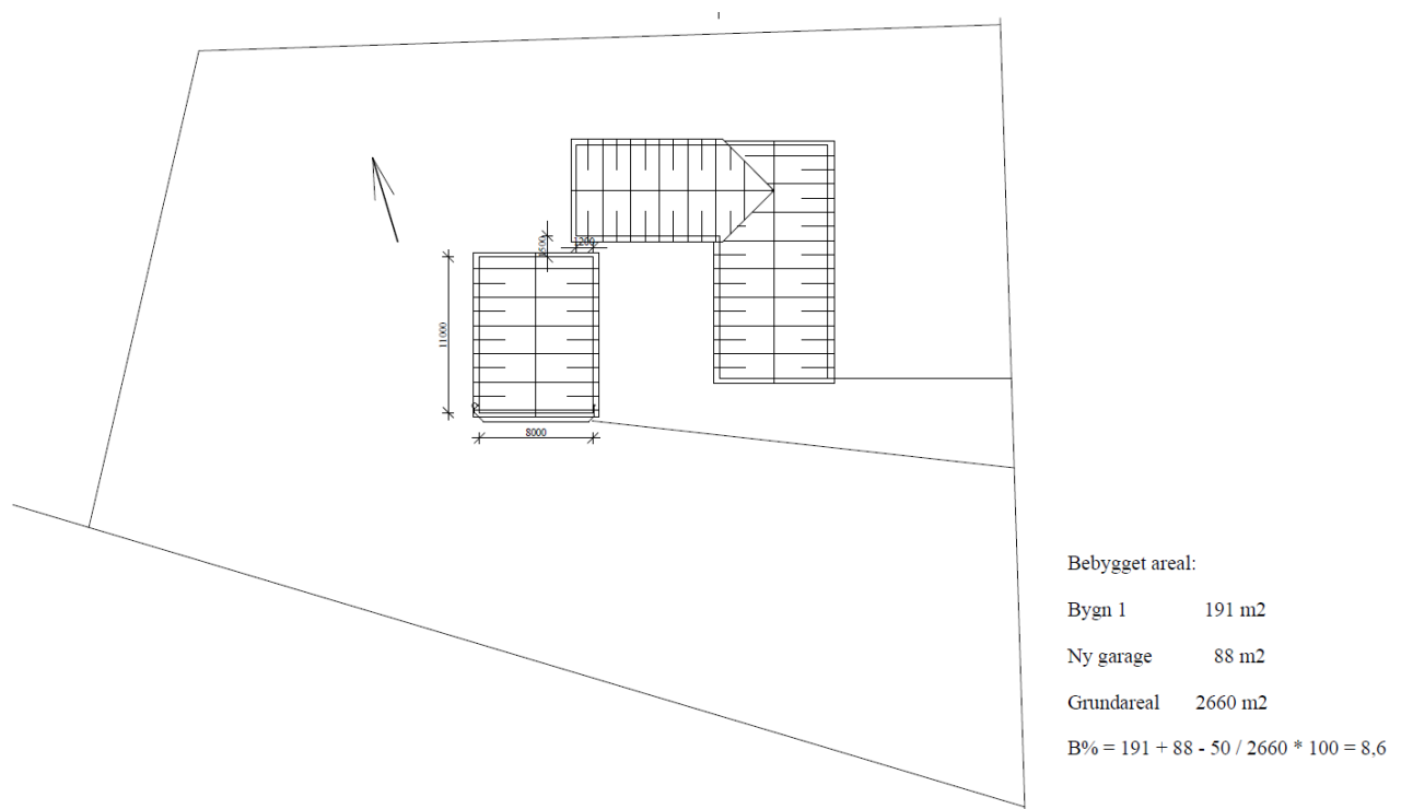
Figur 1. Situationsplan
